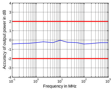
Output power accuracy in dB versus frequency for the R&S®ZNB26/R&S®ZNB40
