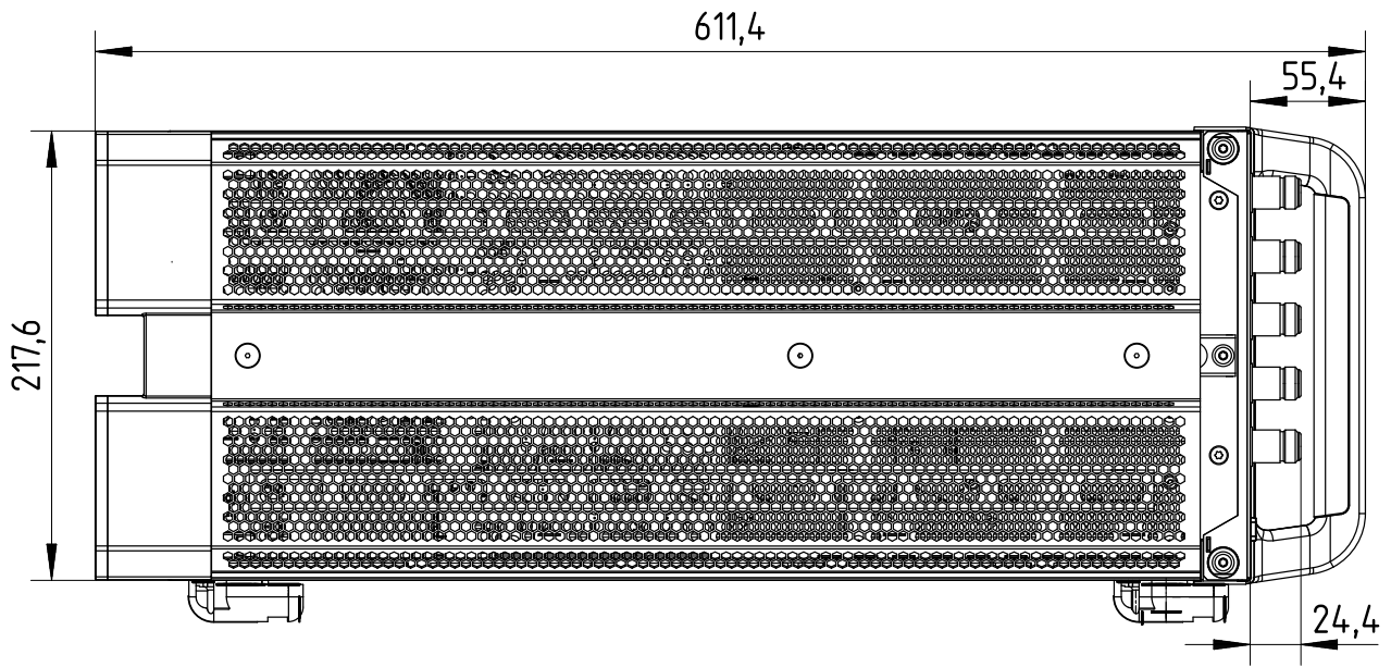
Side view of the R&amp;S®ZNBT8
