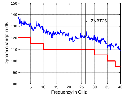
Dynamic range in dB versus frequency for the R&amp;S®ZNBT26/R&amp;S®ZNBT40
