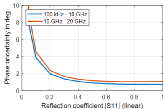
Uncertainty of reflection magnitude and reflection phase measurements for the R&S®ZNBT20 in the frequency range from 100 kHz to 20 GHz; analysis conditions: S_{12} = S_{21} = 0 , cal. power –10 dBm, meas. power –10 dBm
