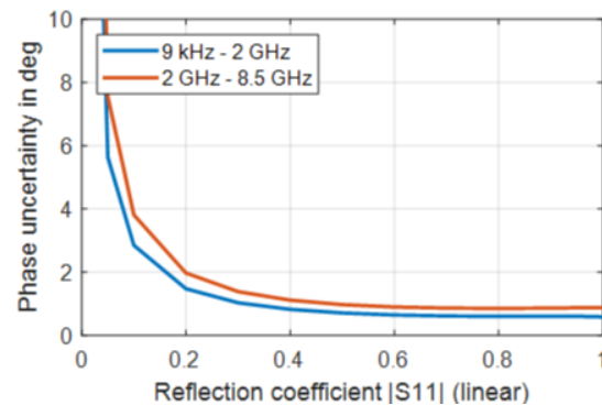
Uncertainty of reflection magnitude and reflection phase measurements for the R&S®ZNBT8 in the frequency range from 9 kHz to 8.5 GHz; analysis conditions: S_{12} = S_{21} = 0 , cal. power –10 dBm, meas. power –10 dBm
