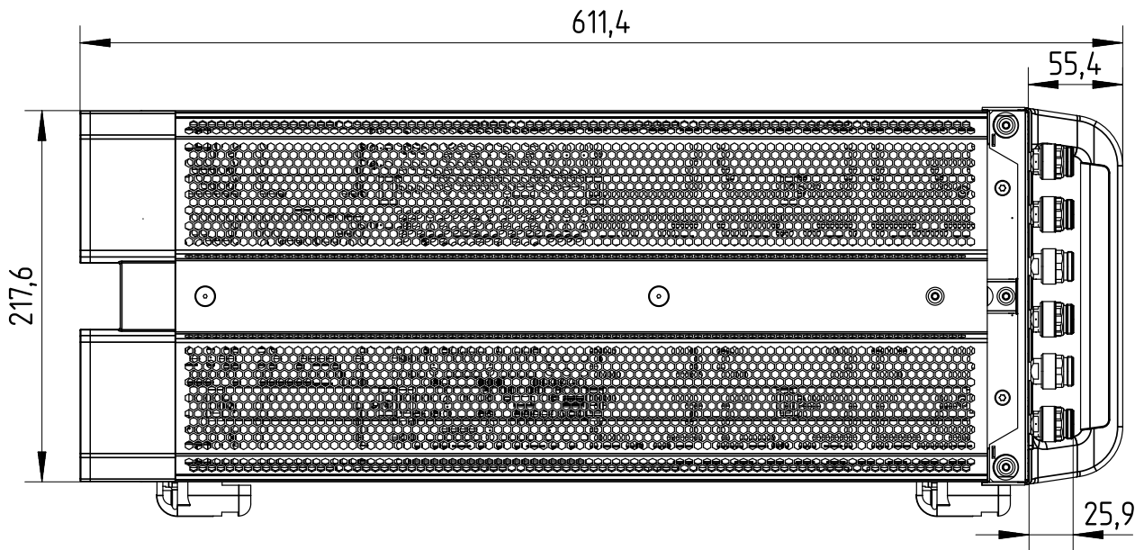
Side view of the R&amp;S®ZNBT20, R&amp;S®ZNBT26 and R&amp;S®ZNBT40
