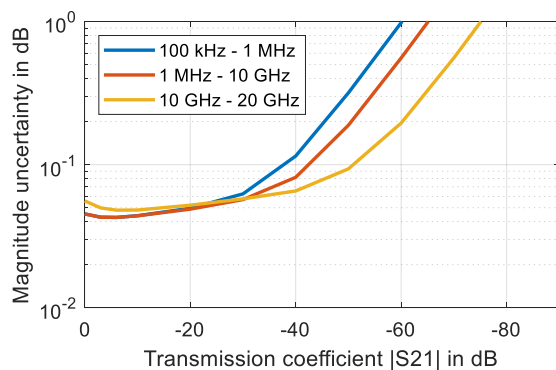
Uncertainty of transmission magnitude and transmission phase measurements for the R&S®ZNBT20 in the frequency range from 100 kHz to 20 GHz; analysis conditions: S_{11} = S_{22} = 0 , cal. power –10 dBm, meas. power –10 dBm
